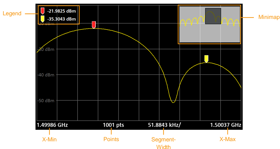
Fig. 5-18 Preview
