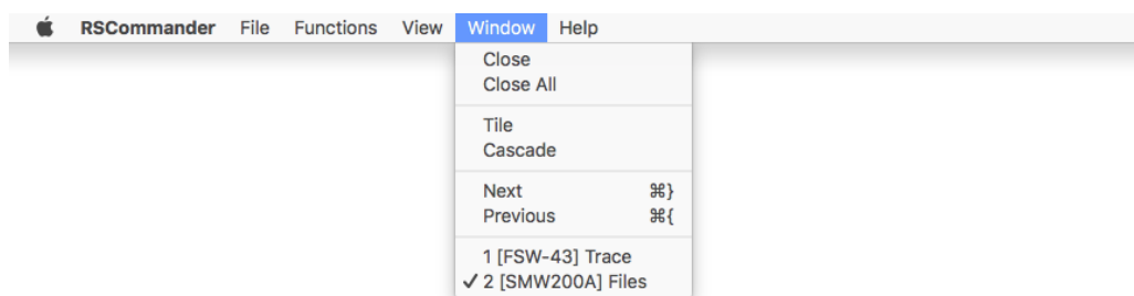
Fig. 5-10: Window Menu
