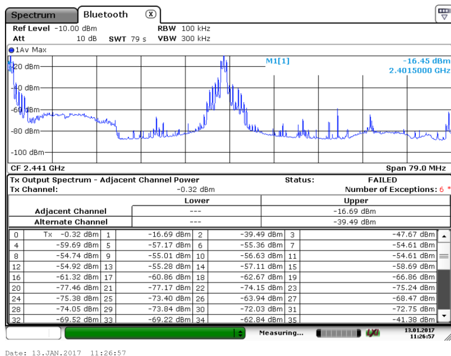
Fig. 4-4: FSV hardcopy
