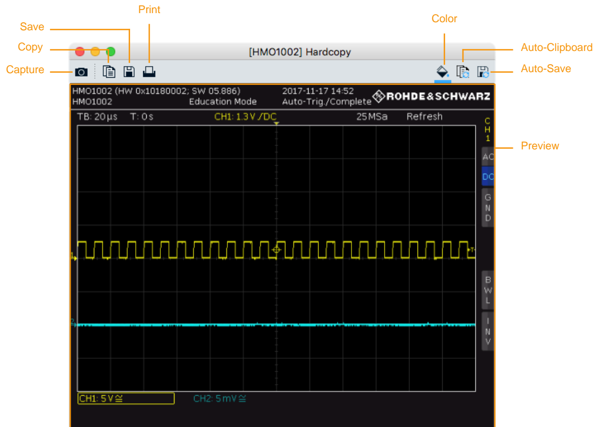
Fig. 5-14: Hardcopy Window
