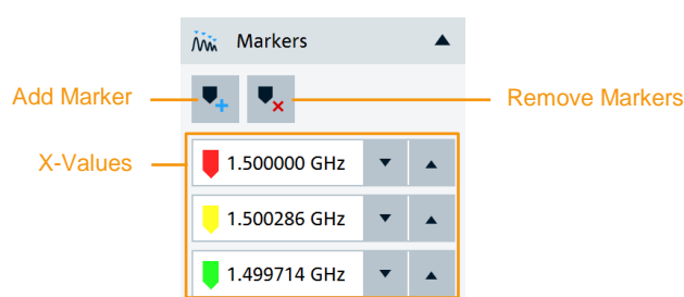
Fig. 5-17 Markers Panel
