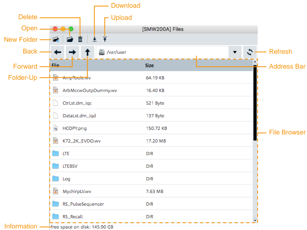
Fig. 5-19: Files Window
