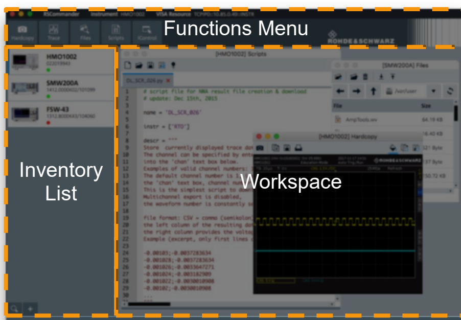
Fig. 5-1 Main Screen
