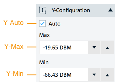
Fig. 5-16 Y-Configuration Panel
