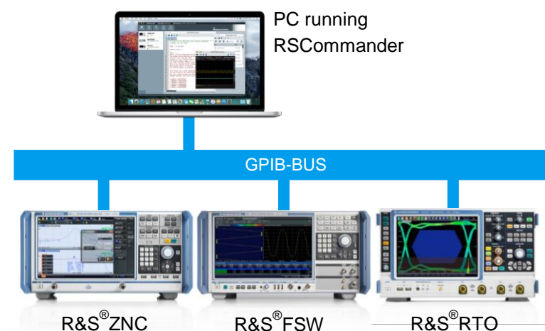
Fig. 3-1: GPIB Instruments
