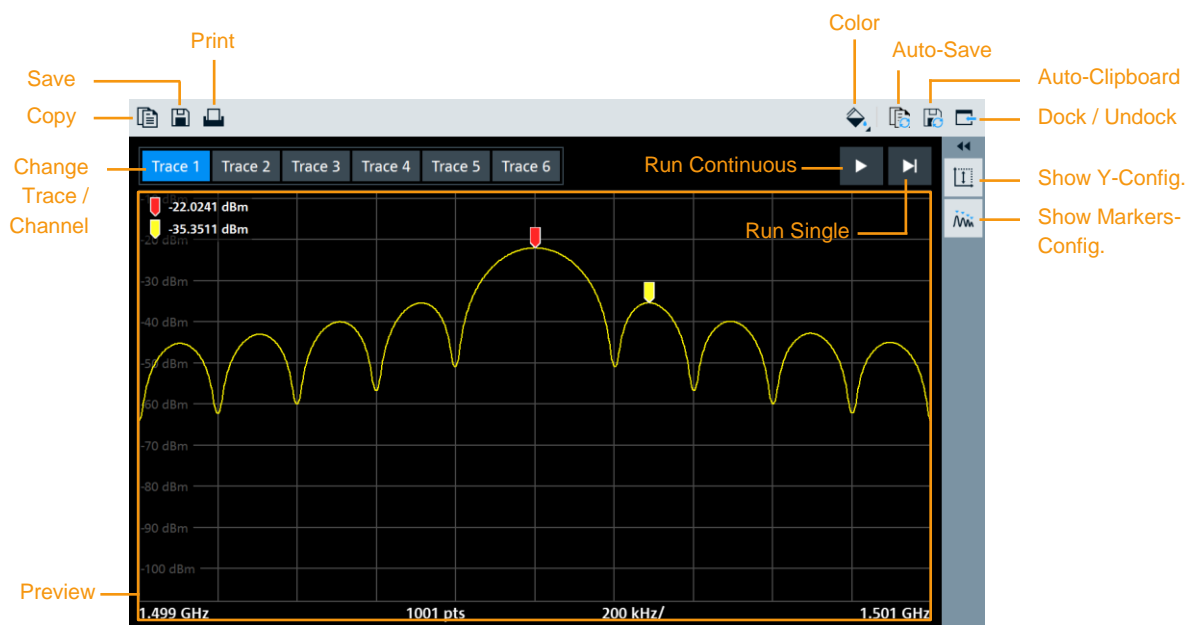
Fig. 5-15: Trace Window
