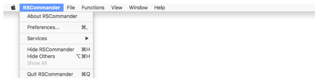
Fig. 5-5: RSCommander Menu
