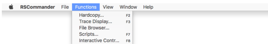
Fig. 5-8: Functions Menu
