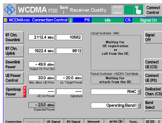
Fig. 5-20: CMU Hardcopy
