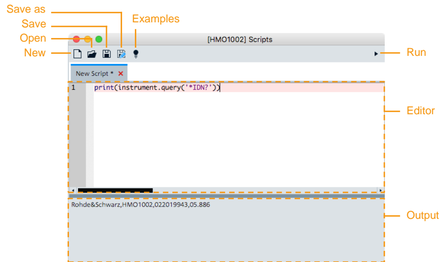
Fig. 5-21: Scripts window
