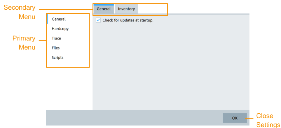
Fig. 5-28: Settings window
