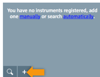
Fig. 4-2: Inventory panel
