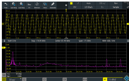
R&S®RTB2000: 10.1" display, 1280 × 800 pixel resolution
