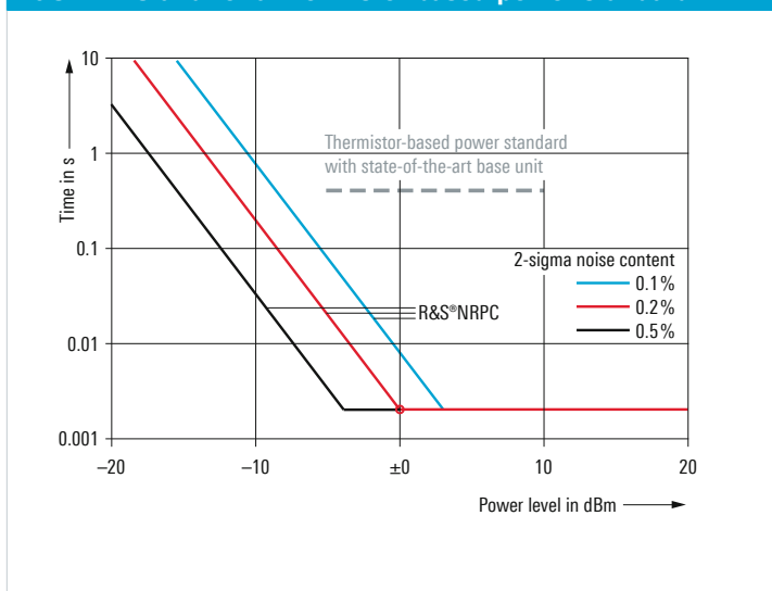
Achievable measurement times per frequency point for the R&S®NRPC and for a thermistor-based power standard
