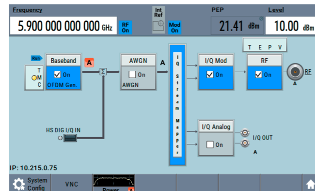
Functional block diagram of the R&S®SMBV100B
