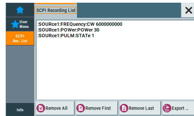
The built-in SCPI macro recorder and code generator support fast, easy generation of SCPI sequences
