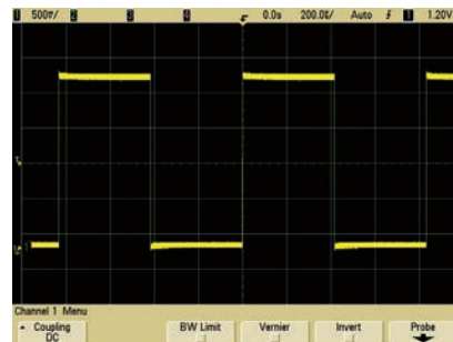
Properly compensated
