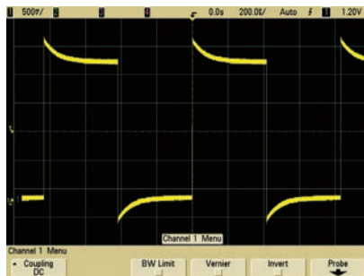
Over-compensated
