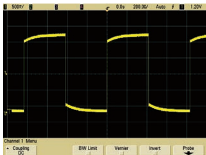
Under-compensated
