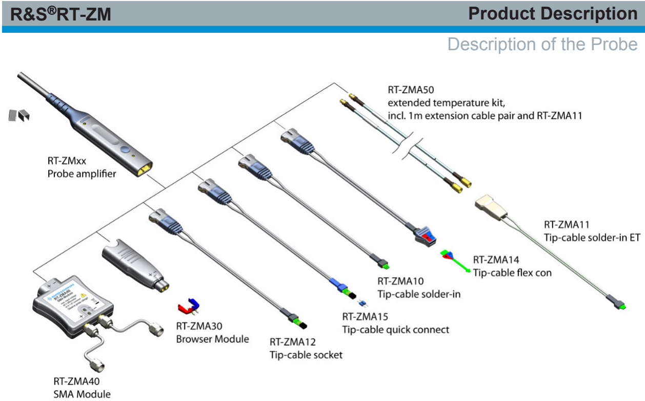
Figure 1-2: R&S RT-ZM probing system compatibility chart
