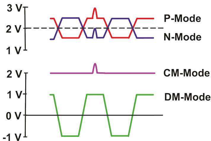
Figure 2-3: Displayed voltage on oscilloscope screen
