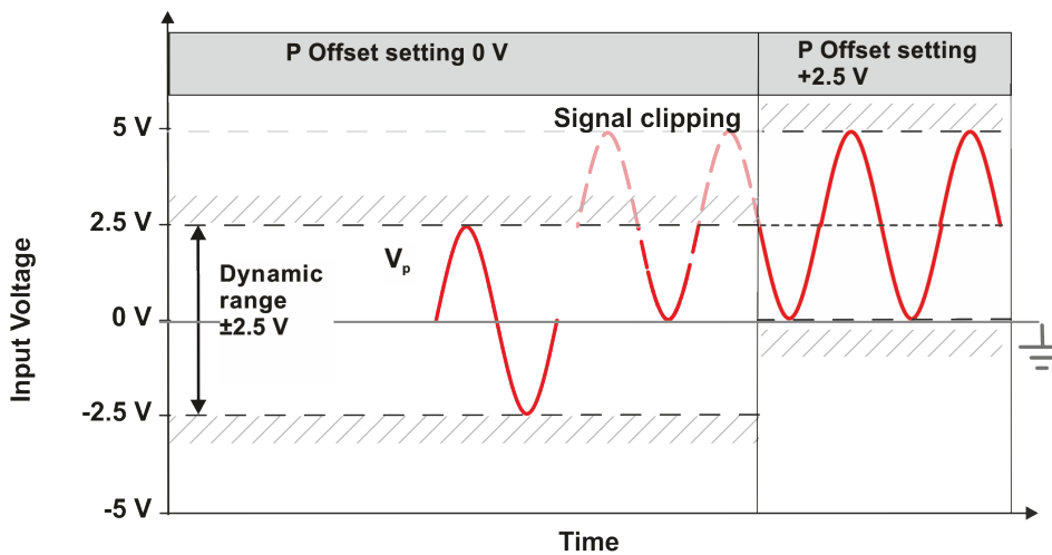
Figure 2-7: P offset compensation for a single-ended measurement at the positive input terminal
