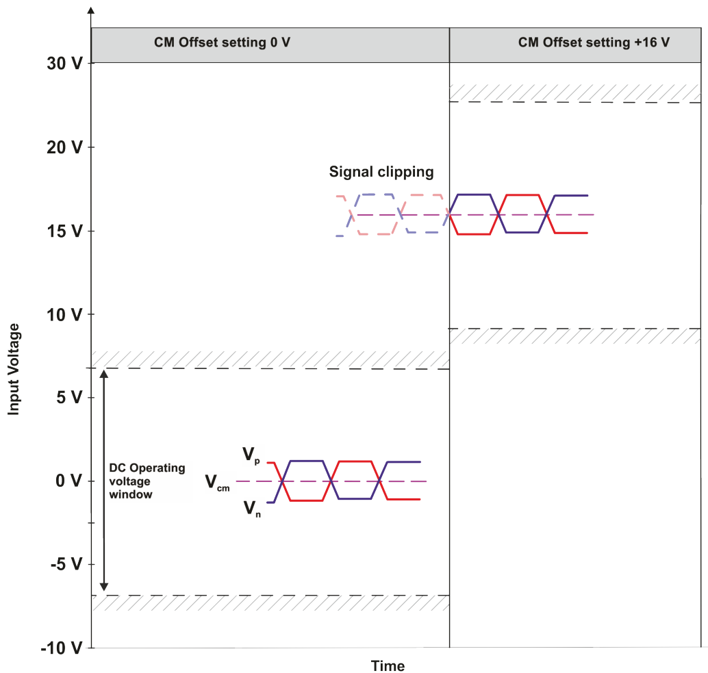
Figure 2-6: Common mode (CM) offset compensation for a differential measurement
