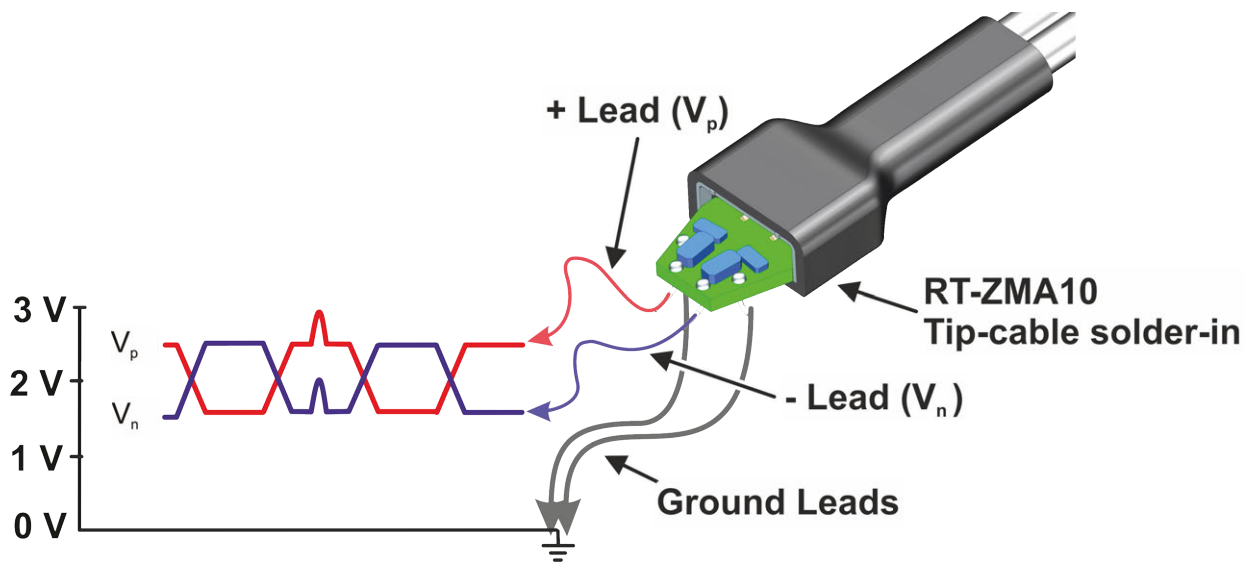
Figure 2-2: Input voltage at probe tip
