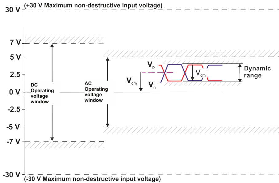
Figure 2-4: Operating voltage window for differential measurement mode DM at 10:1 attenuation for all offset settings at 0 V
