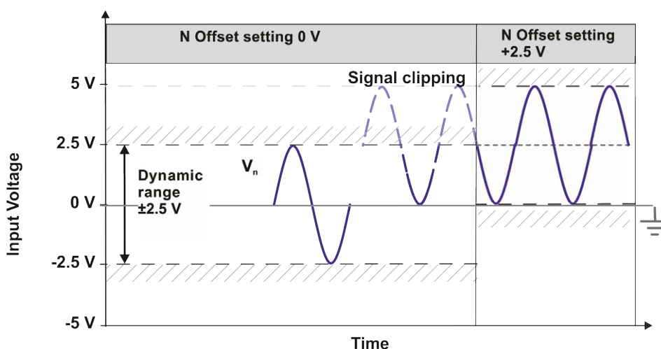
Figure 2-8: N offset compensation for a single-ended measurement at the negative input terminal
