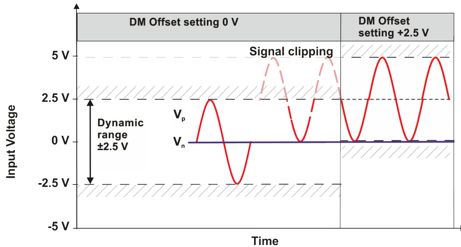
Figure 2-5: Differential offset compensation for a single-ended measurement (negative input connected to ground) using an R&S RT-ZM15/30/60/90/130/160
