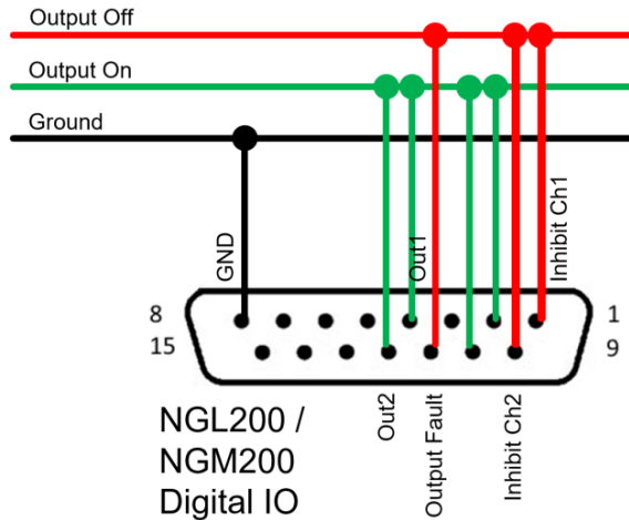
Figure 3-1 Connection schematic of the digital IO connectors
