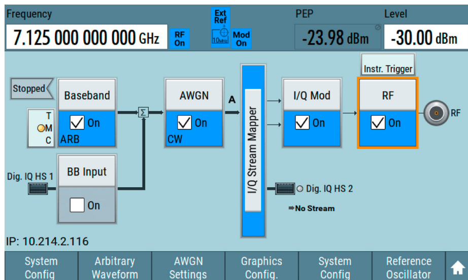
R&amp;S®SMCV100B graphical user interface with block diagram
