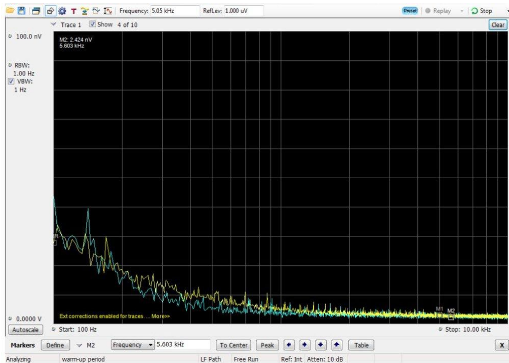
Figure 28: Input referred Noise Density 100nV full scale, mid-range noise density is 2nV/Root-Hz.
