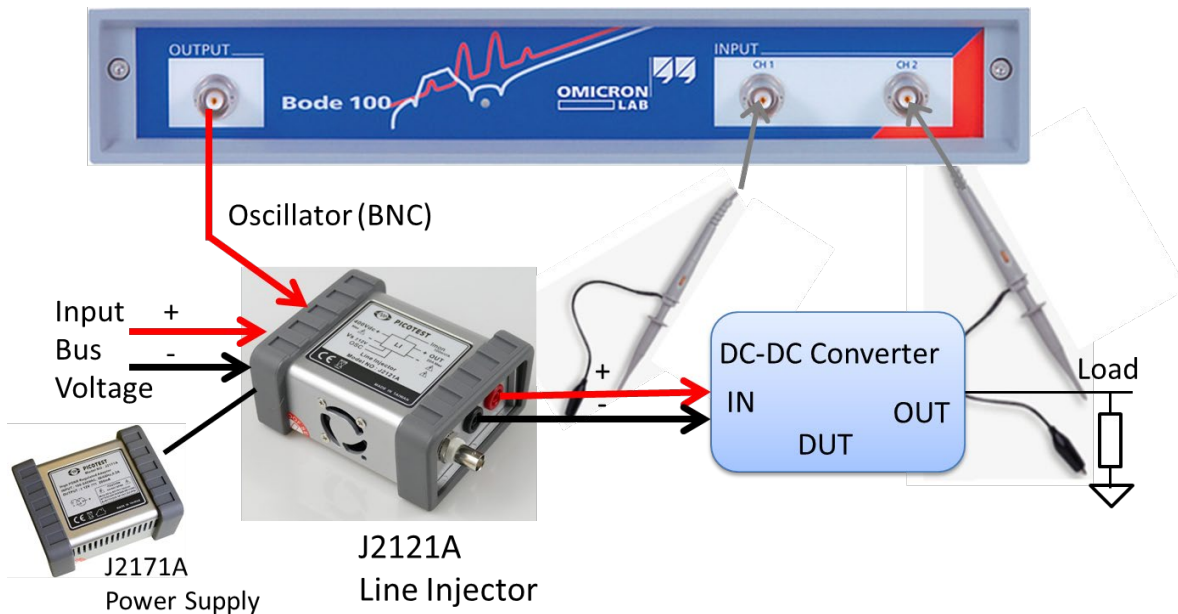
Figure 15: J2121A Line Injector Connections for PSRR measurements.
