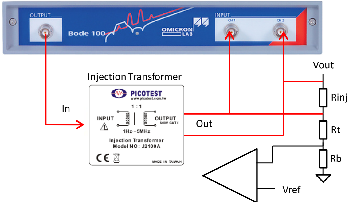
Figure 7: Injection Transformer Connections for stability measurements.
