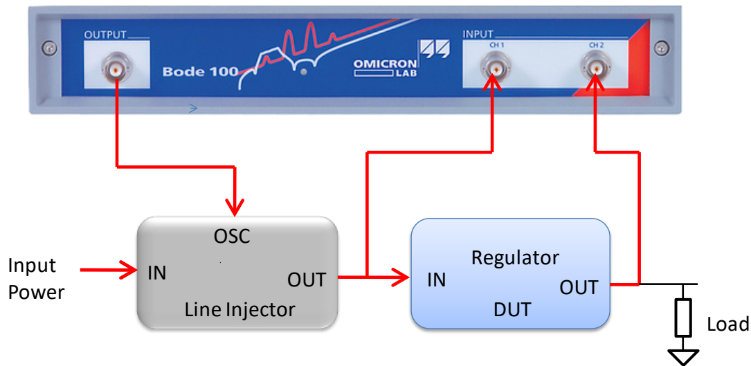
Figure 11: Line Injector Connections for PSRR measurements.
