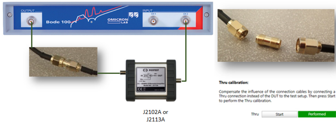
Figure 37: Calibrating the 2-Port Shunt-Through Measurement. The J2102A has been replaced by the J2102B.
