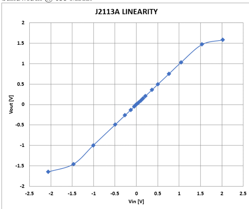
Figure 45: J2113A Linearity Graph.
