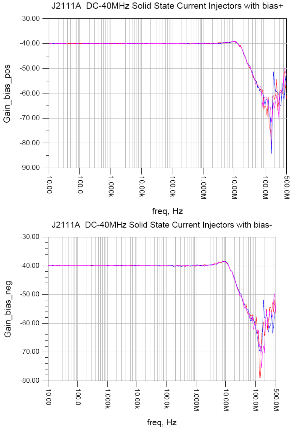
Figure 24: J2111A frequency response.
