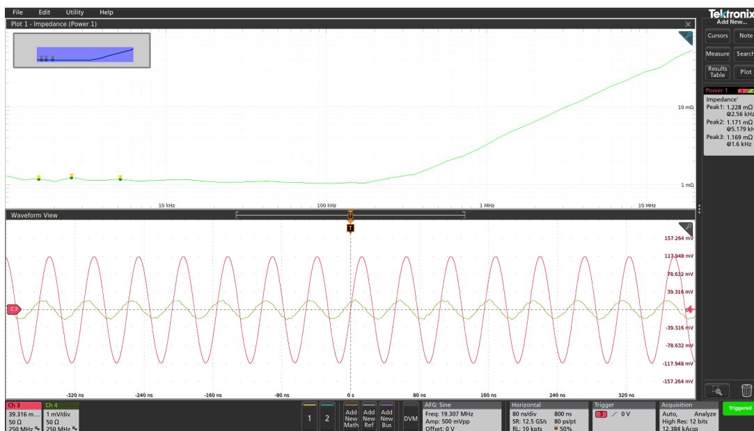
Figure 48: 2-Port Shunt-Thru Impedance measurement of a 1m Ohm (1.17m) resistor.
