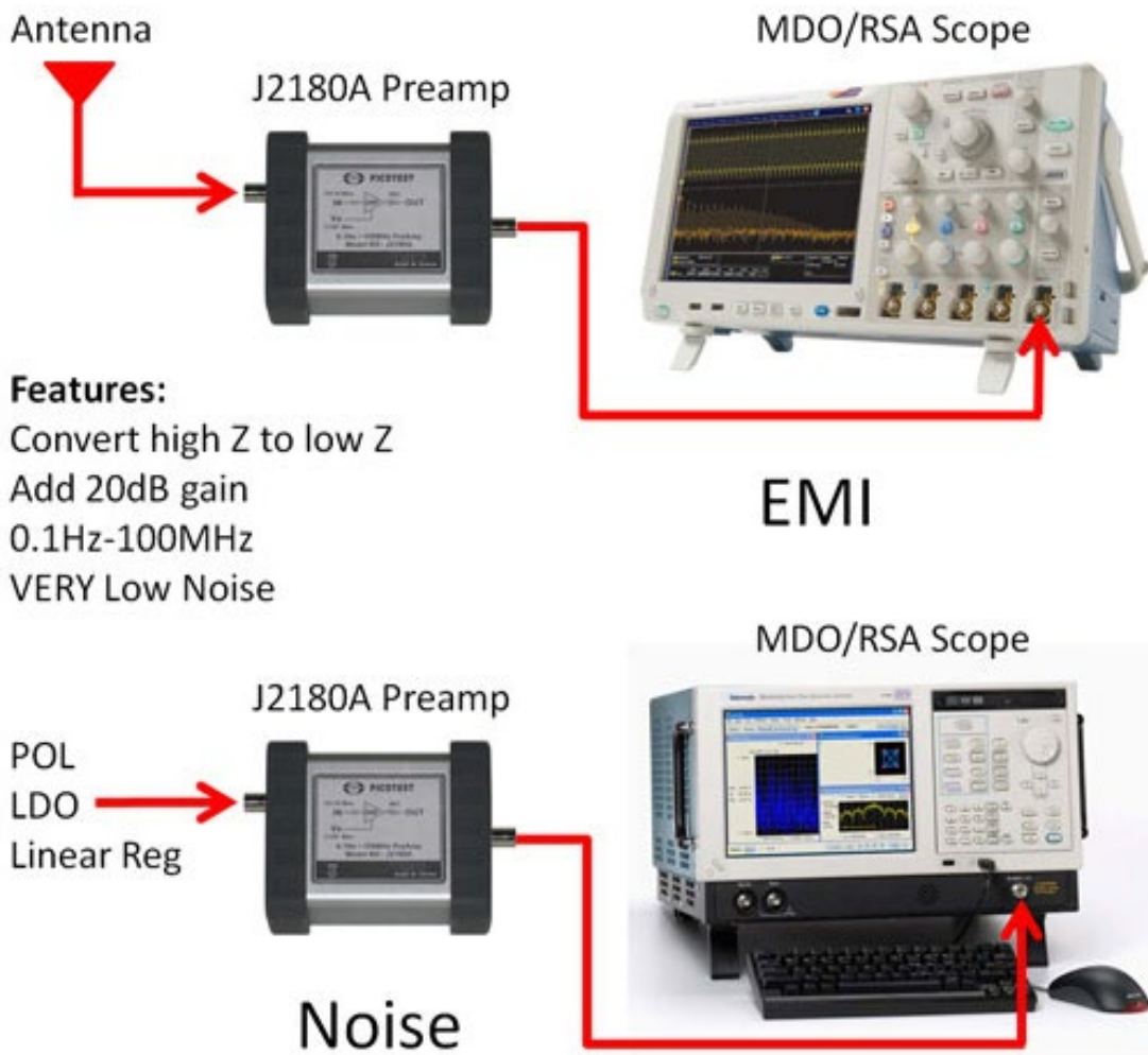
Figure 27: Sample setups for the J2180A Preamp used for noise and EMI measurements.
