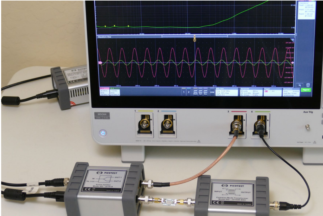
Figure 47: – Tektronix Series 6 test setup to perform the 2-port shunt-through impedance measurement using the Picotest J2161A active splitter (left) and the J2102B common mode transformer (right).
