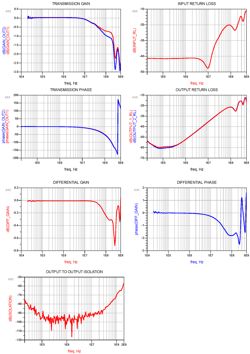
Figure 52: J2161A Typical measured frequency response data.
