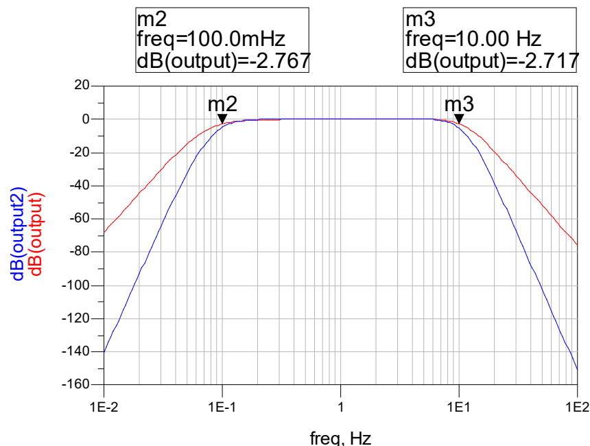
Figure 29: Frequency response of a single filter (red trace) and 2 cascaded filters (blue trace).
