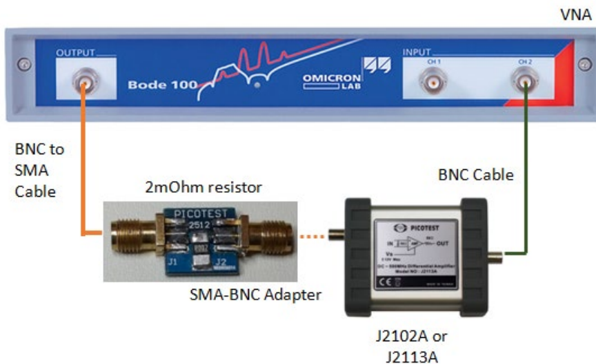
Figure 38: Measuring a low value resistor. The J2102A has been replaced by the J2102B.
