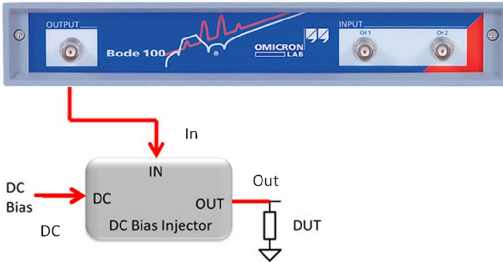
Figure 18: Connections for DC Bias Impedance measurements.
