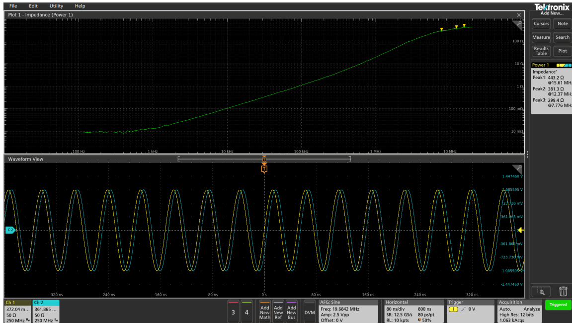
Figure 50: 2-Port Shunt-Thru Impedance measurement of a 3.3uH inductor.
