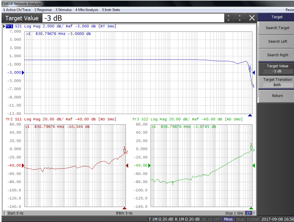
Figure 44: S21, S11, and S22 plots show 3dB S21 -3dB bandwidth @ 830MHz and S22 -6dB bandwidth @ 635 MHz.
