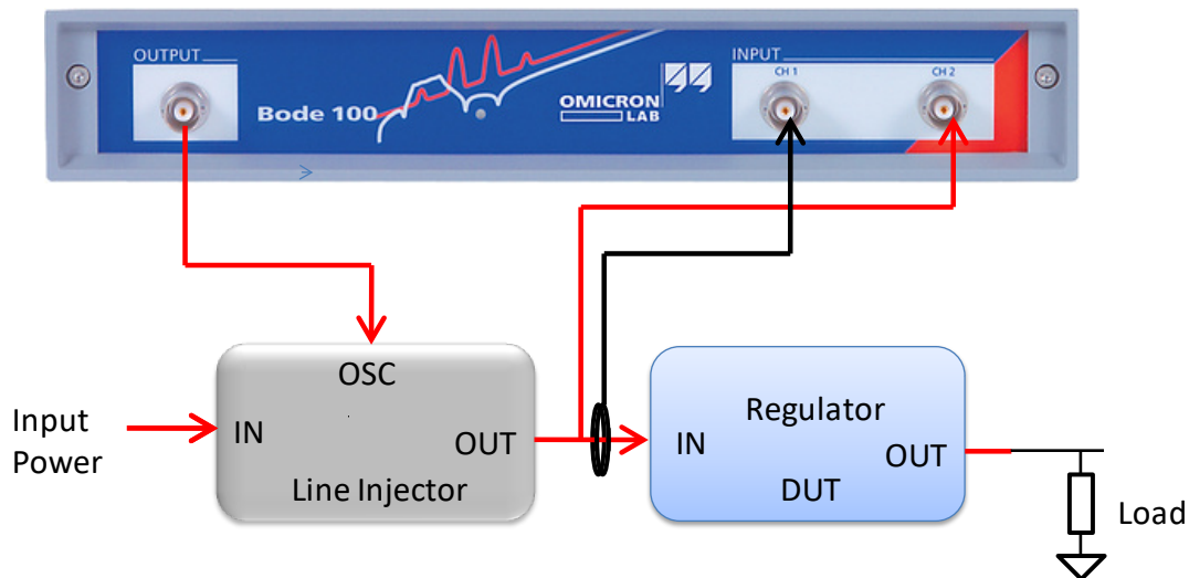
Figure 12: Line Injector Connections for input impedance measurements.
