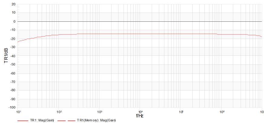
Figure 9: Frequency Response for J2101A injection transformer.
