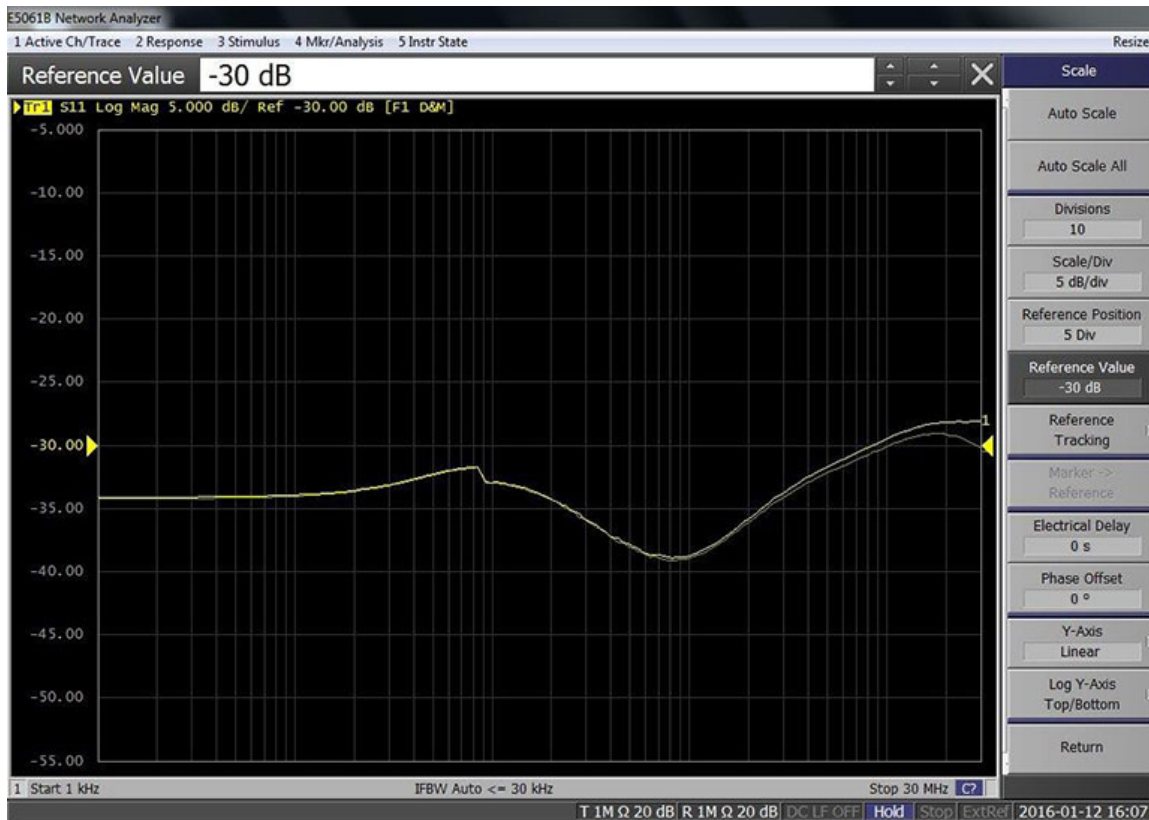
Figure 60: The return loss of the 6dB splitter legs is better than 25dB over the full measurement range of the instrument.
