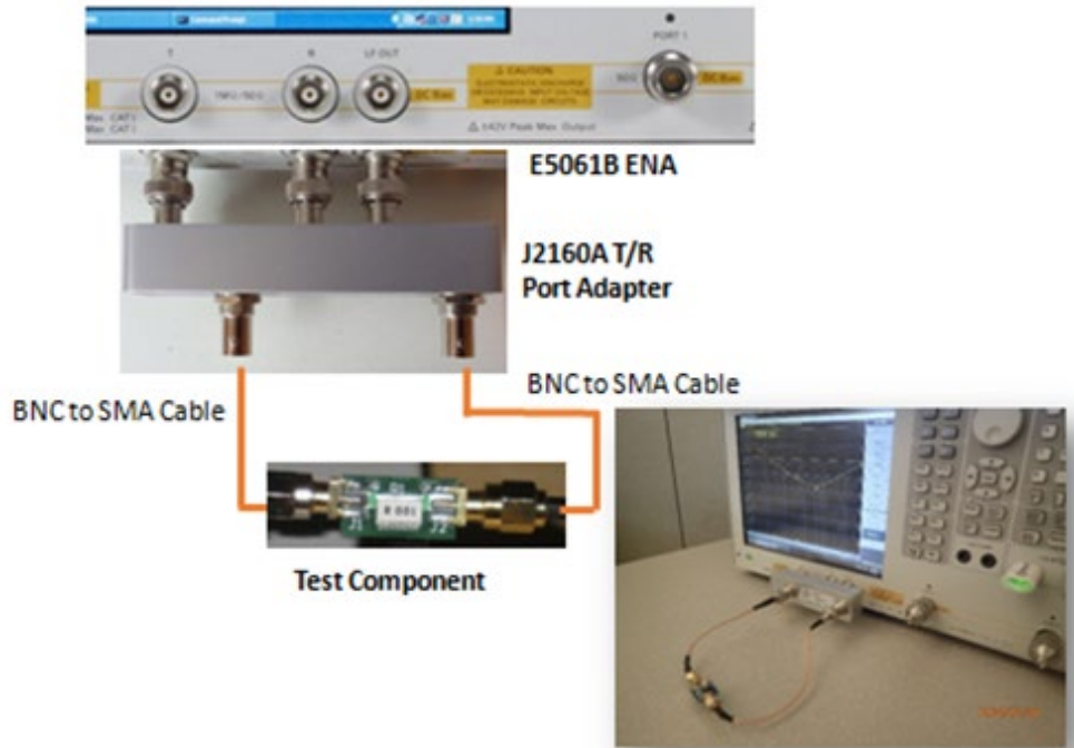
Figure 55: Measuring Components Using the Keysight E5061B GP Ports (Low Frequency).
