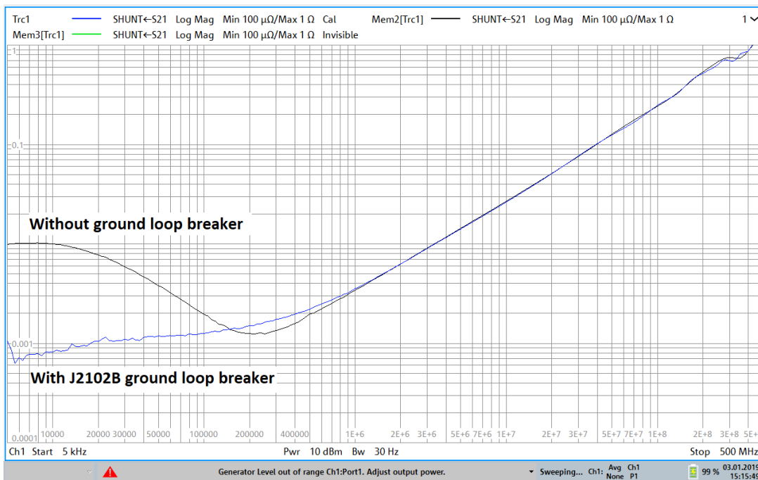
Figure 34: Impedance measurement of a 1mΩ resistor with and without the J2102B common mode transformer using the Rohde & Schwarz ZNL VNA.
