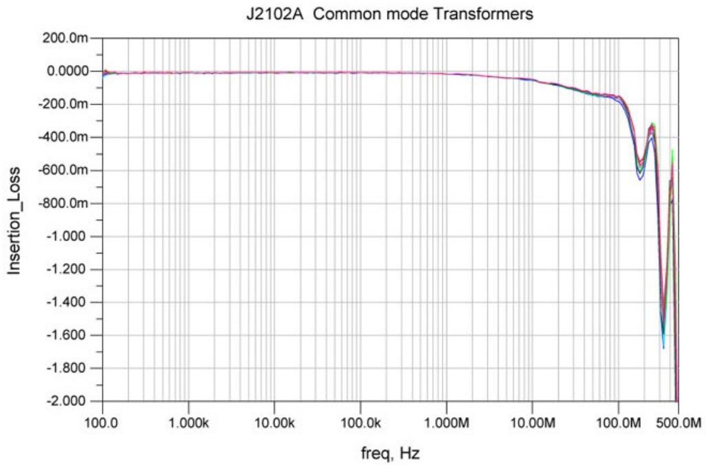
Figure 36: J2102A Insertion Loss Graph.
