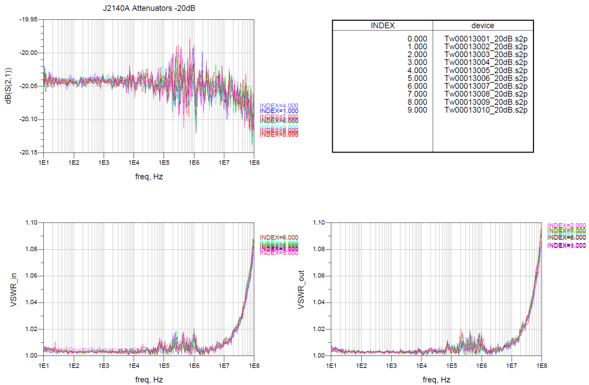
Figure 26: J2140A S21 and VSWR frequency response.
