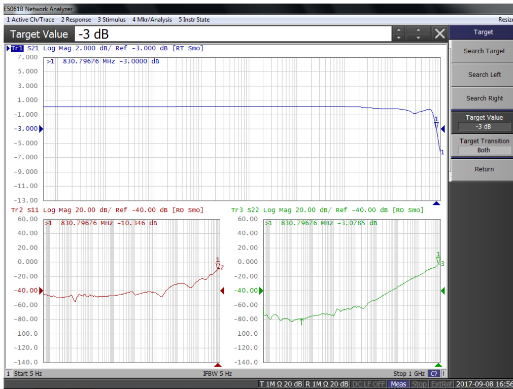
Figure 51: S21, S11, and S22 plots show 3dB S21 -3dB bandwidth @ 830MHz and S22 -6dB bandwidth @ 635 MHz.
