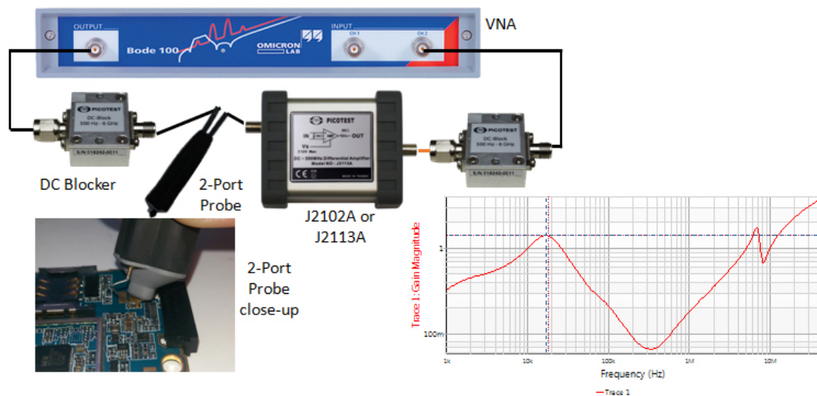
Figure 40: Measuring the in-circuit output impedance using the Picotest P2101A 2-Port Transmission Line Probe. The J2102A has been replaced by the J2102B.
