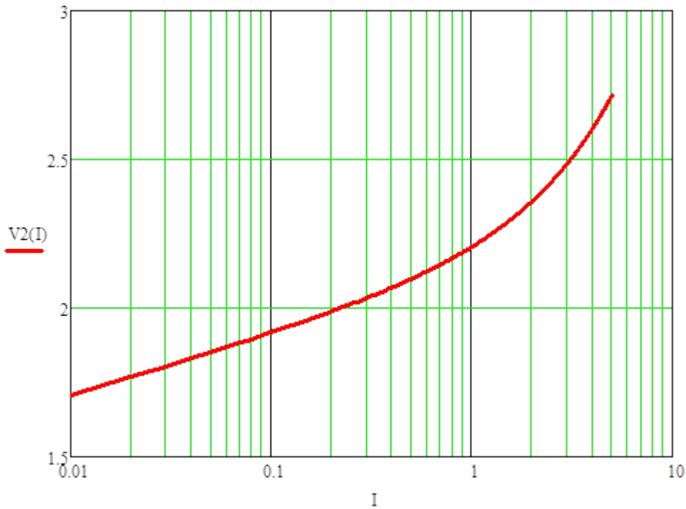
Figure 13: Line Injector voltage drop.
