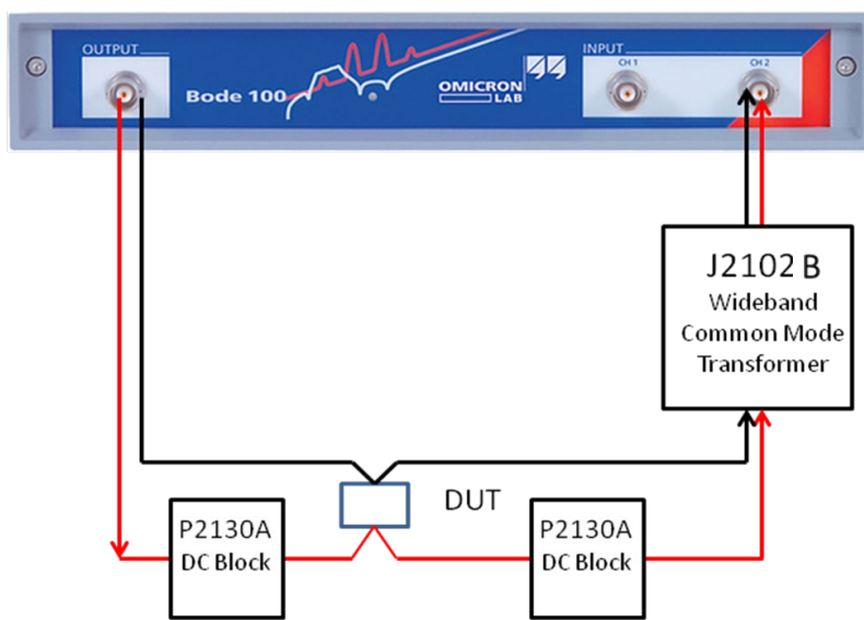
Figure 30: Connection diagram showing the placement of the J2102B common mode transformer. Inclusion of the transformer eliminates the low frequency distortion caused by instrumentation ground loops.
