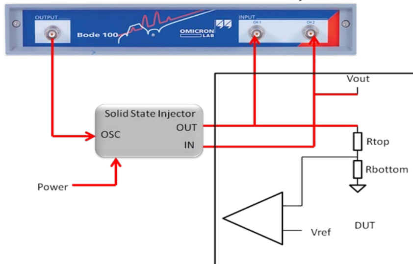
Figure 10: Solid-State Injector Connections for stability measurements.
