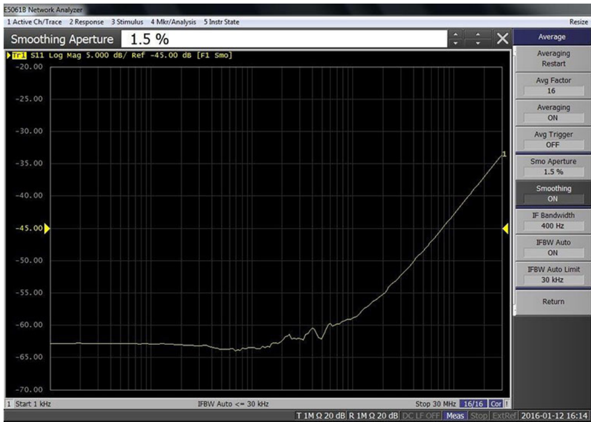
Figure 58: The T port return loss is better than 30dB over the full frequency range of the instrument.
