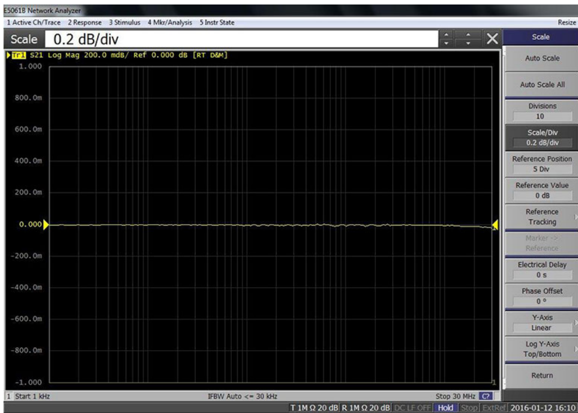
Figure 59: The T port insertion loss is less than a few hundredths of a dB over the full instrument range.
