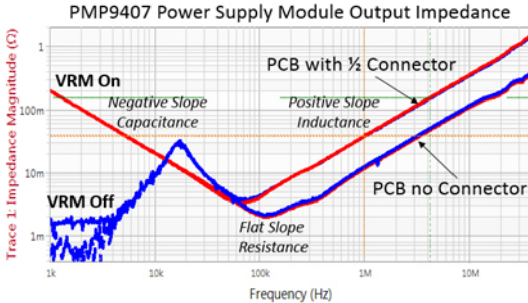
Figure 43: 2-Port Shunt-Thru Impedance measurement results using two 1-Port PDN Probes.
