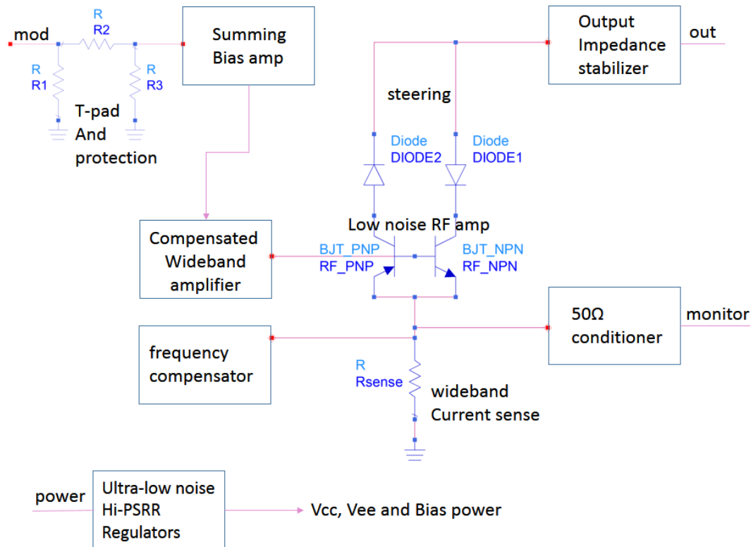
Figure 22: Current Injector internal block diagram.
