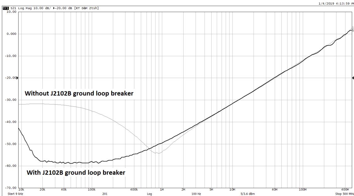
Figure 33: Impedance measurement of a 1mΩ resistor with and without the J2102B common mode transformer using the Copper Mountain S5065 VNA.
