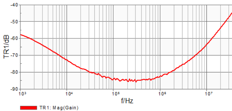
Figure 32: Common Mode Frequency response of the J2102B.
