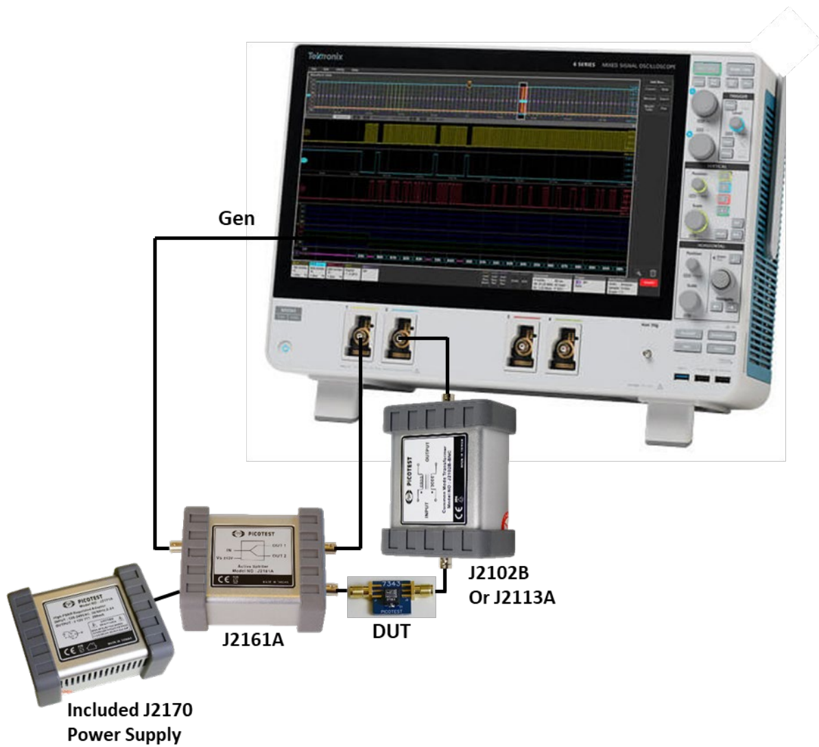
Figure 46: – 2-port shunt through impedance test setup using the Tektronix Series 6 scope, J2161A, and the J2102B.
