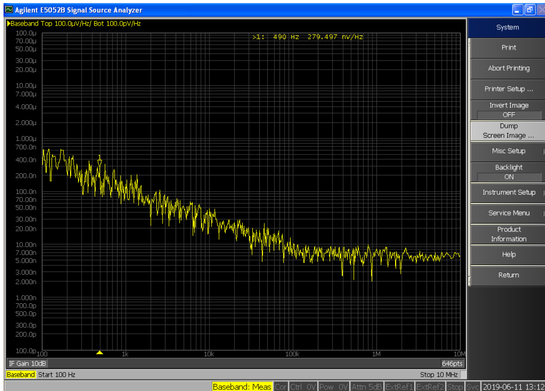
Figure 53: J2161A Typical Noise Density plot.
