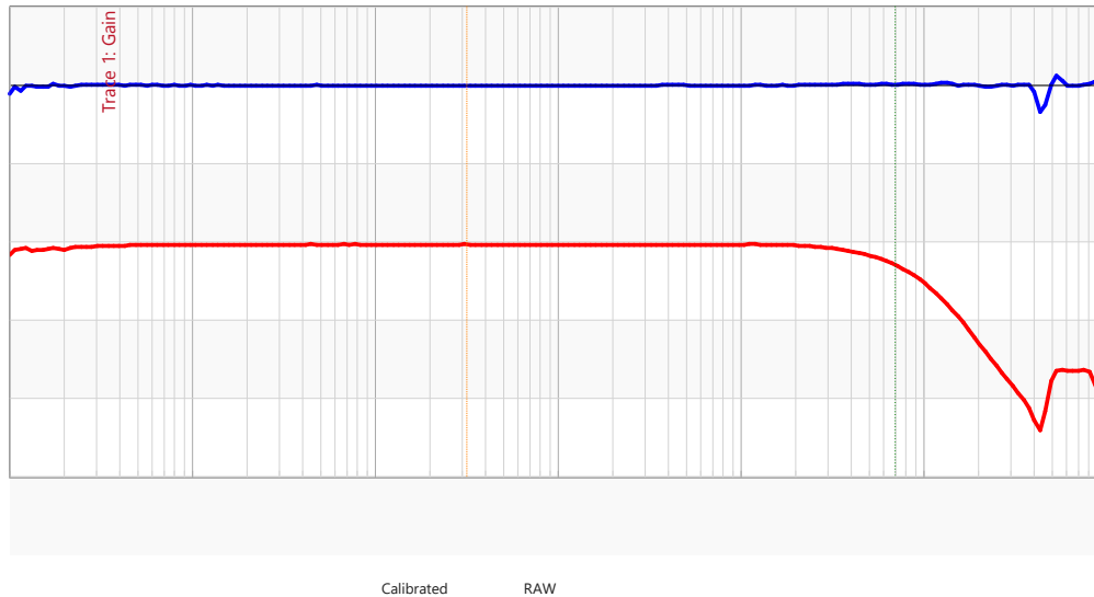
Figure 16: The current monitor transfer ratio measurement shows the 100mV/A (-20dB) transfer function from the modulation current to the current monitor output. Uncalibrated, the -3dB frequency is 700kHz. Calibrated the response is 10Hz-1MHz.
