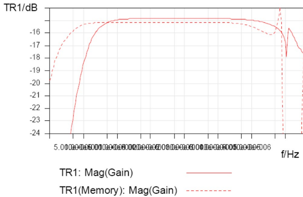
Figure 8: Frequency Response for the J2100A and J2101A injection transformer.
