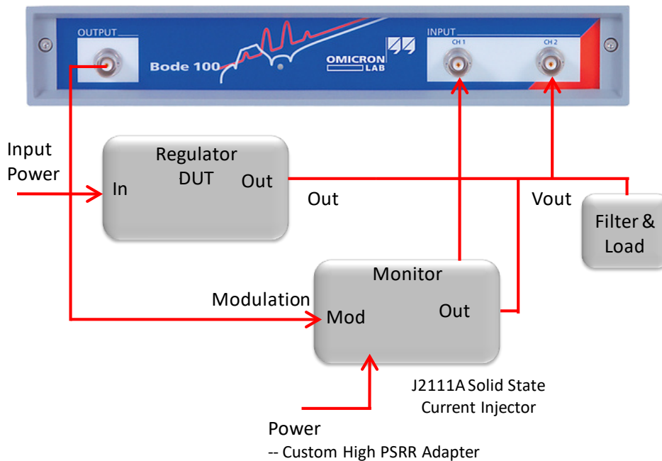
Figure 23: Current Injector Connections for output impedance measurements.
