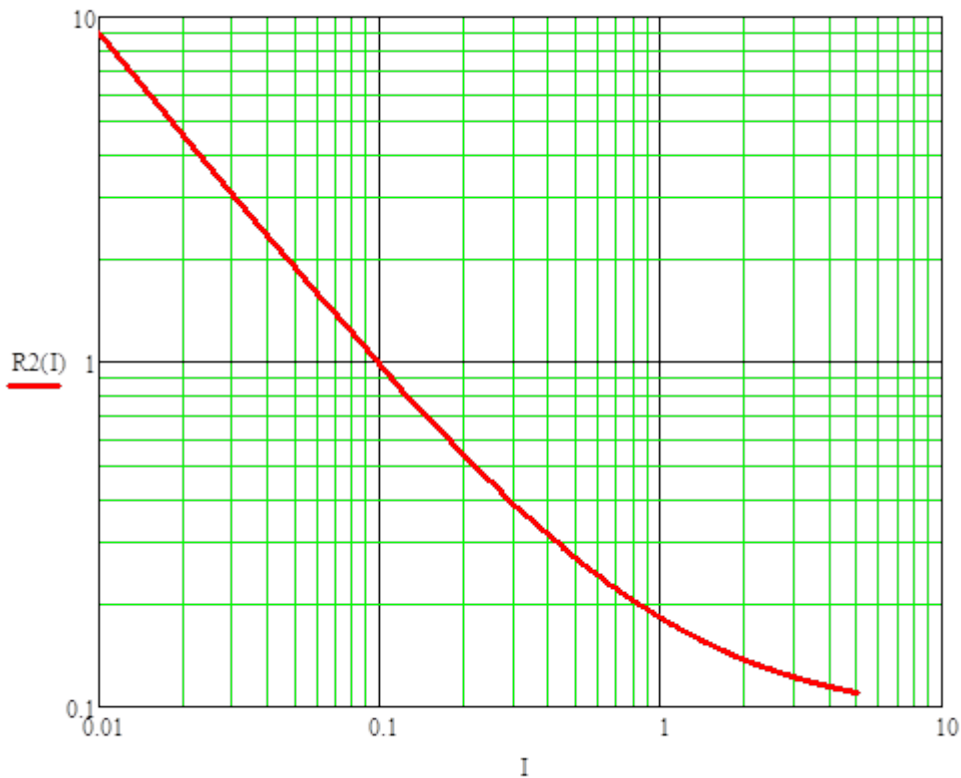
Figure 14: Line Injector output resistance.
