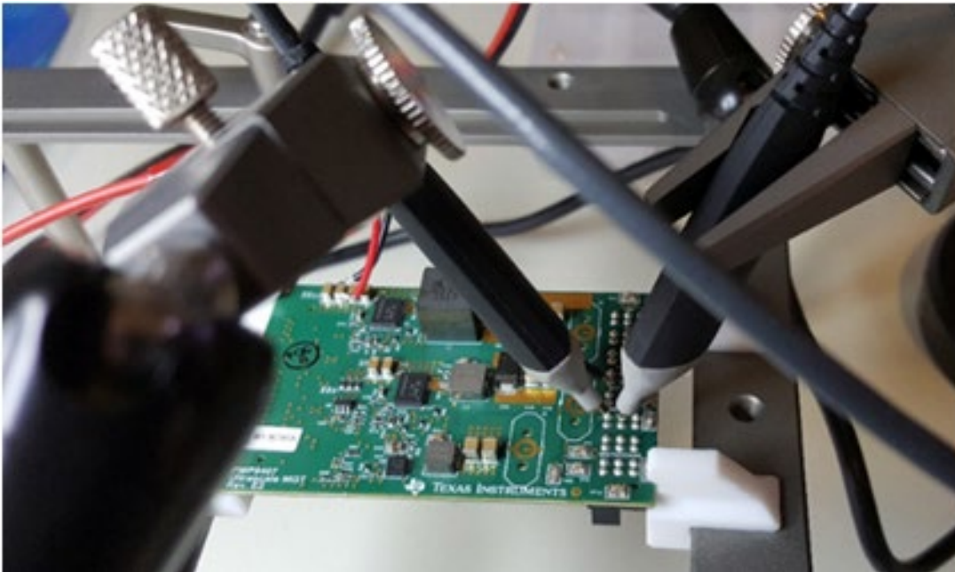
Figure 42: Setup image of the in-circuit 2-port impedance measurement using two 1-Port PDN Probes.
