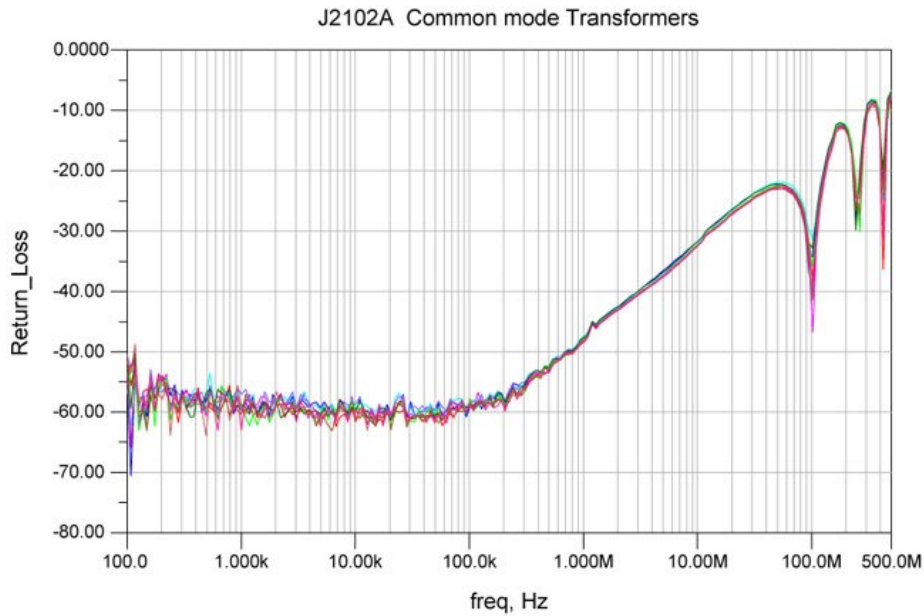
Figure 35: J2102A Return Loss Graph.
