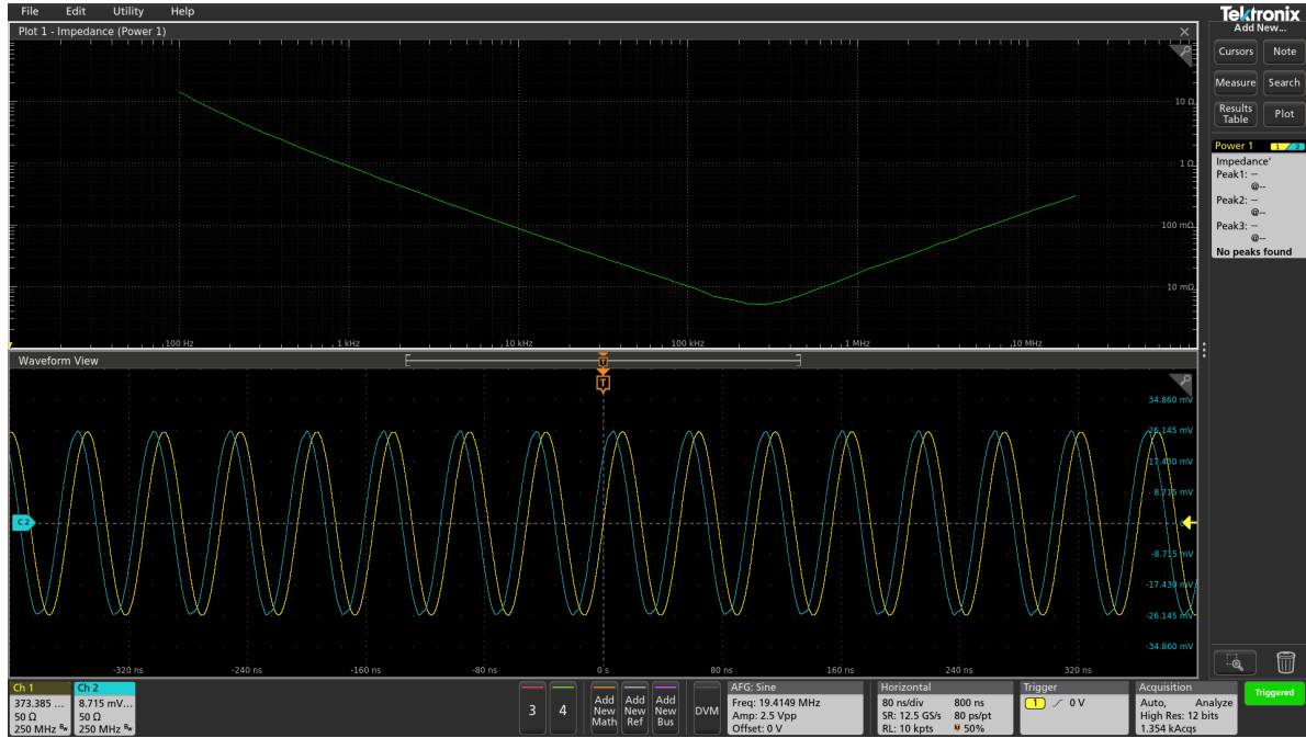
Figure 49: 2-Port Shunt-Thru Impedance measurement of a 100uF polymer capacitor.
