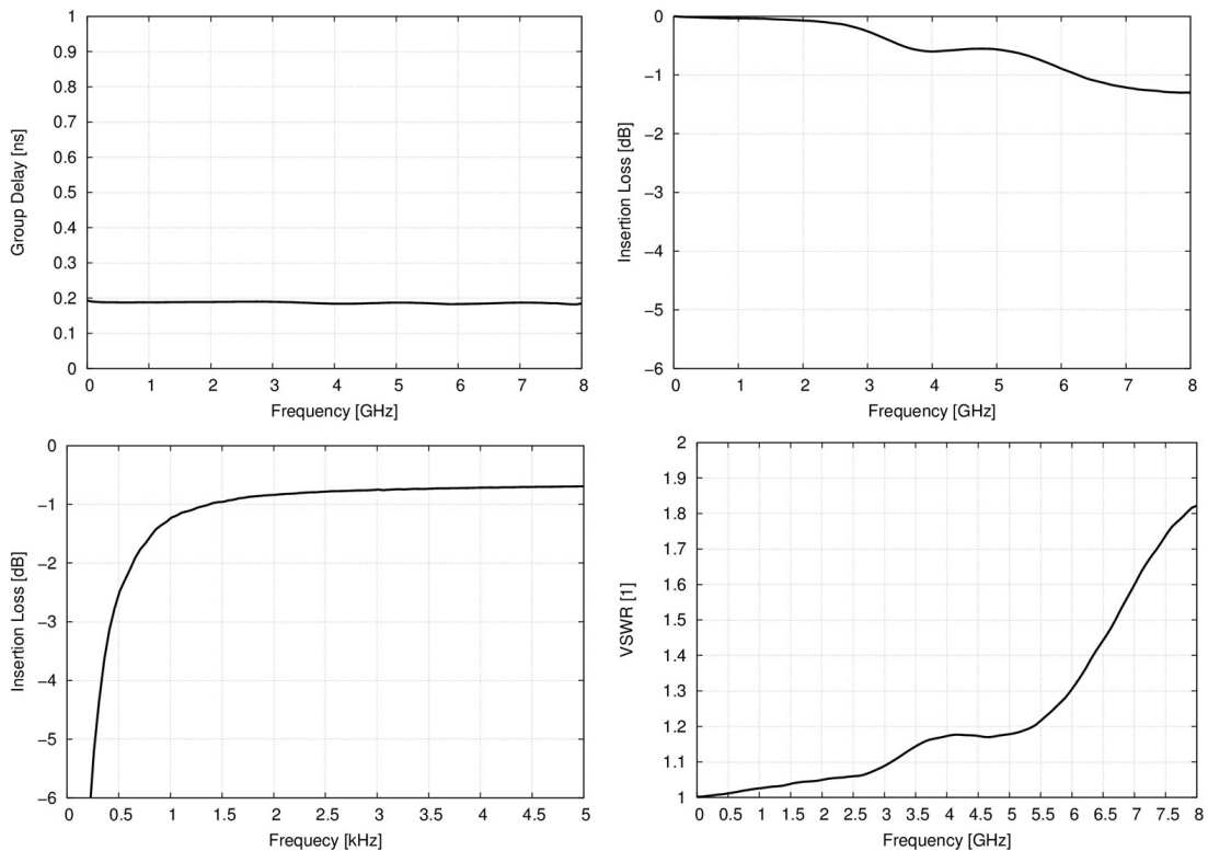
Figure 21: Electrical performance characteristics of the P2130A DC blocker.
