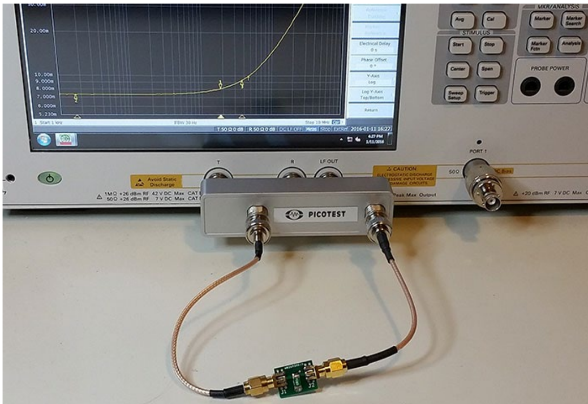
Figure 54: 2 Port Probe Adapter Panel for the Keysight E5061B VNA.
