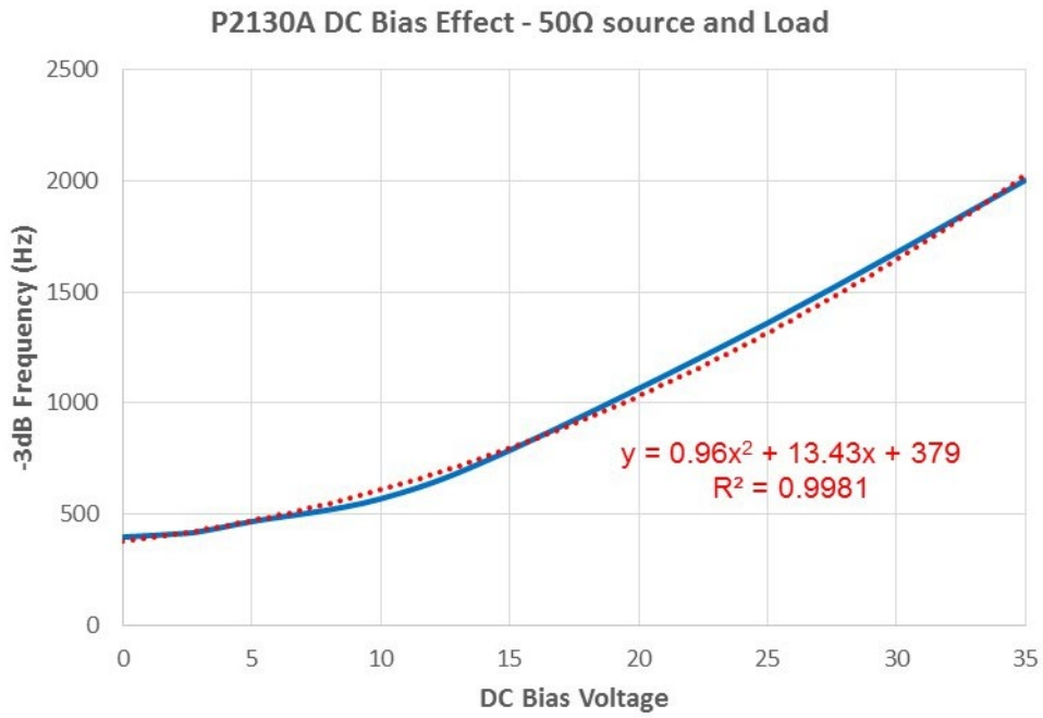
Figure 20: The effect of DC bias on the J2130A and P2130A frequency performance which shifts the - 3dB frequency.
