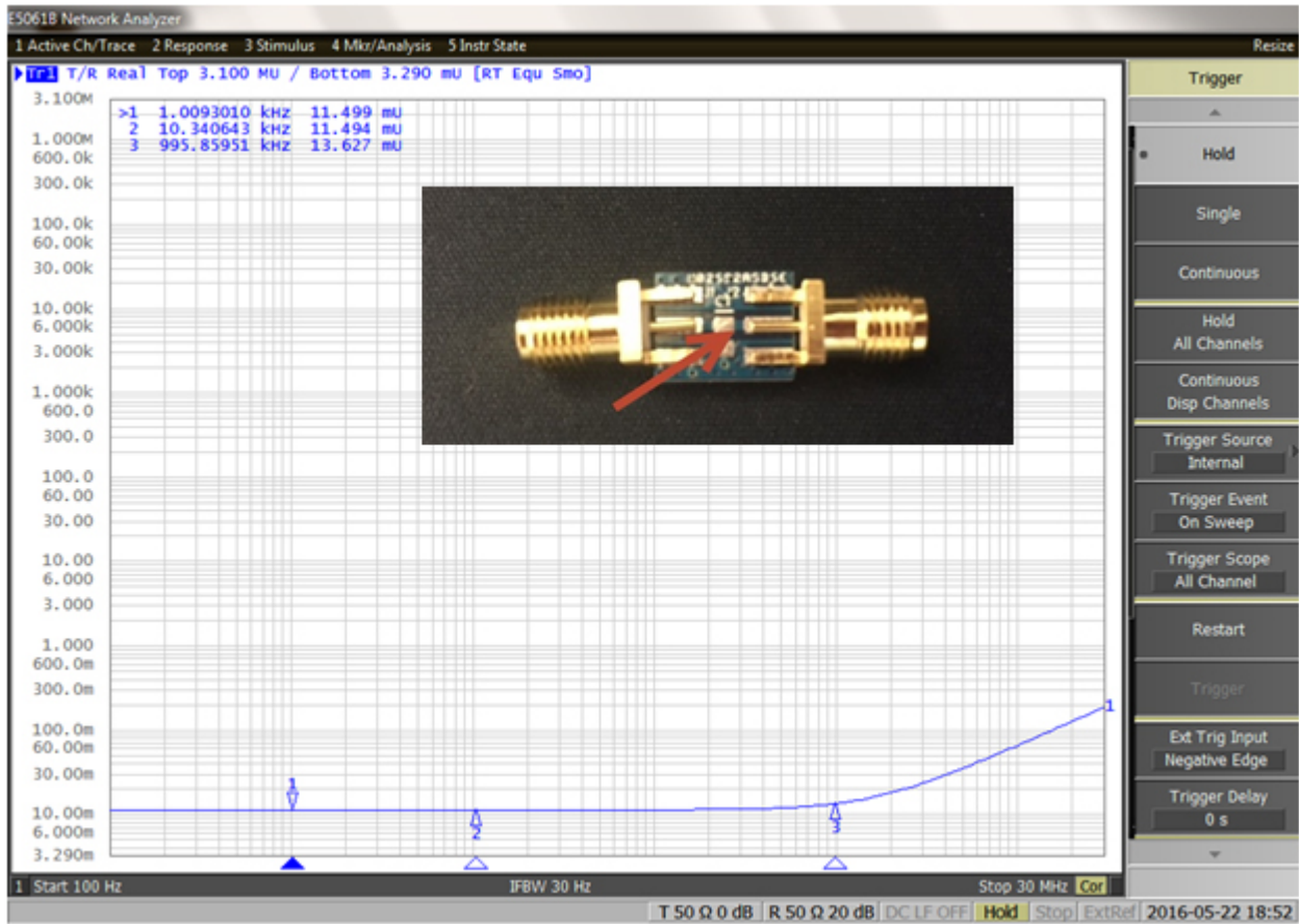
Figure 56: 10 milli-ohm Resistor measurement using the Keysight E5061B VNA GP Ports and the Picotest J2160 adapter.
