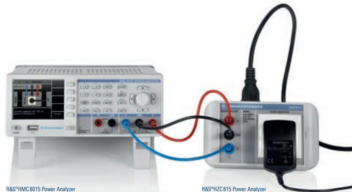
R&amp;S®HMC8015 Power Analyzer
