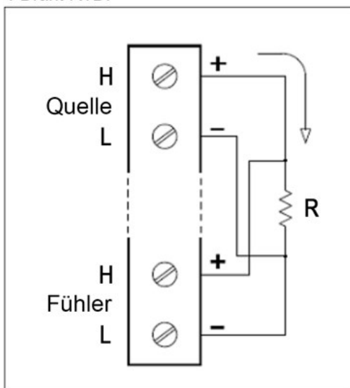
4-Draht-RTD:
