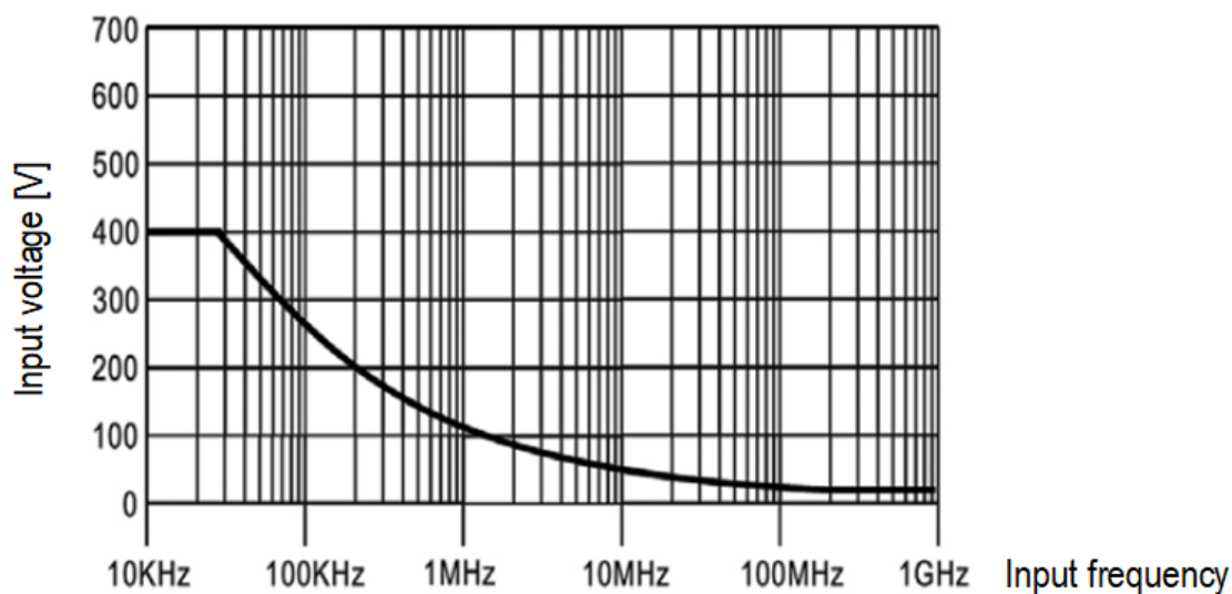
Figure 2-1: Derating curve
