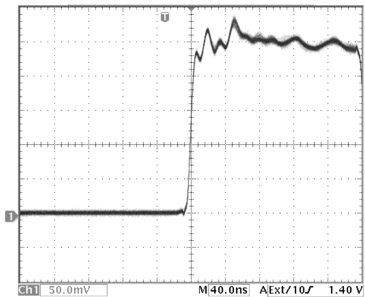
Figure 2 Rise Time
