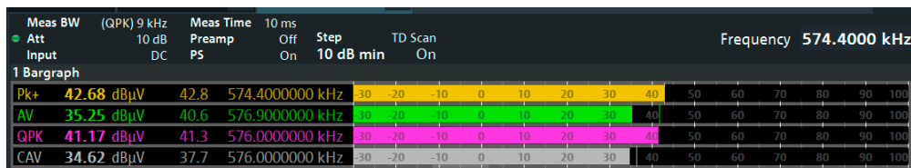
Bargraph display with four detectors.
