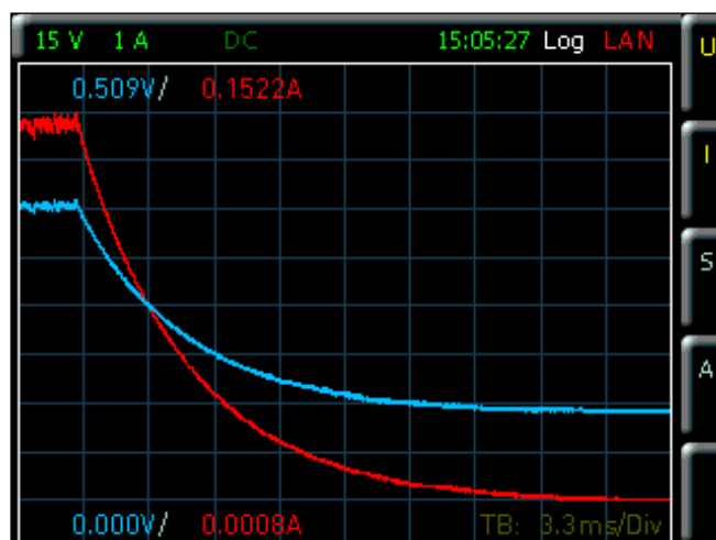
Inrush function
