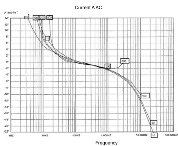
Phase shift according to frequency
