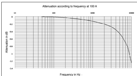
Attenuation according to frequency
