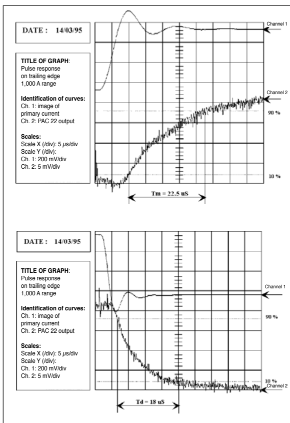
Pulse response
