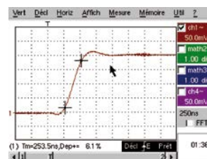
Pulse response
