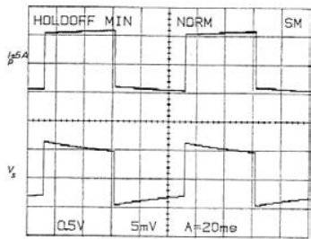
5 A at 500 Hz
