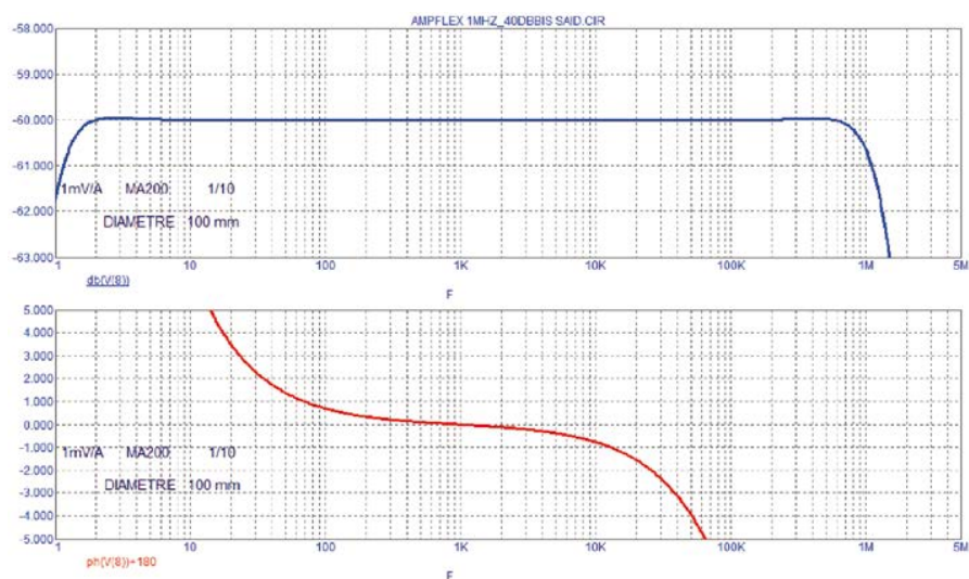
Frequency and phase responses (10)
