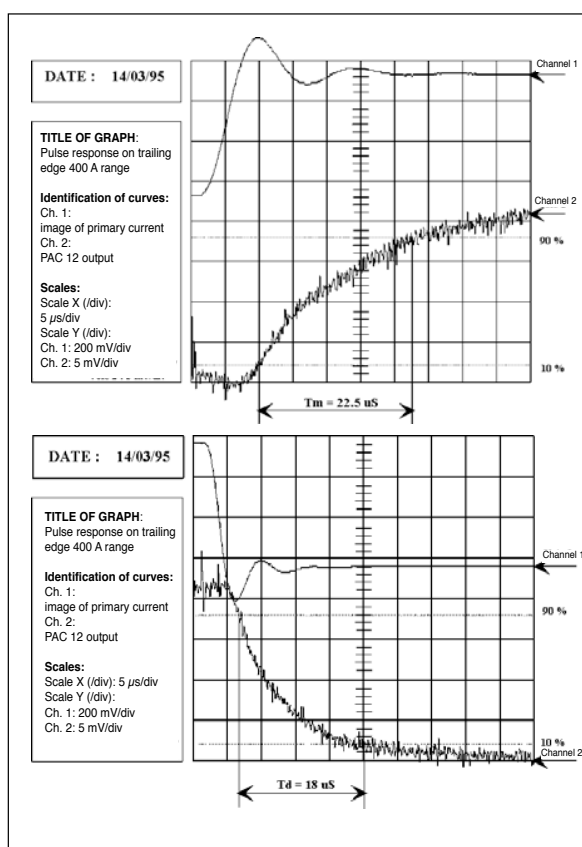
Pulse response
