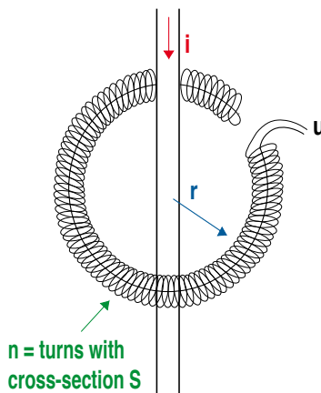
Rogowski coil
