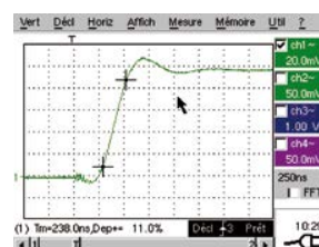
Pulse response
