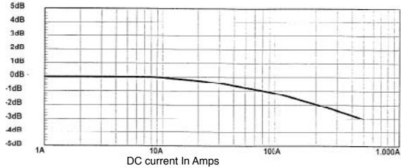
Influence of DC current
