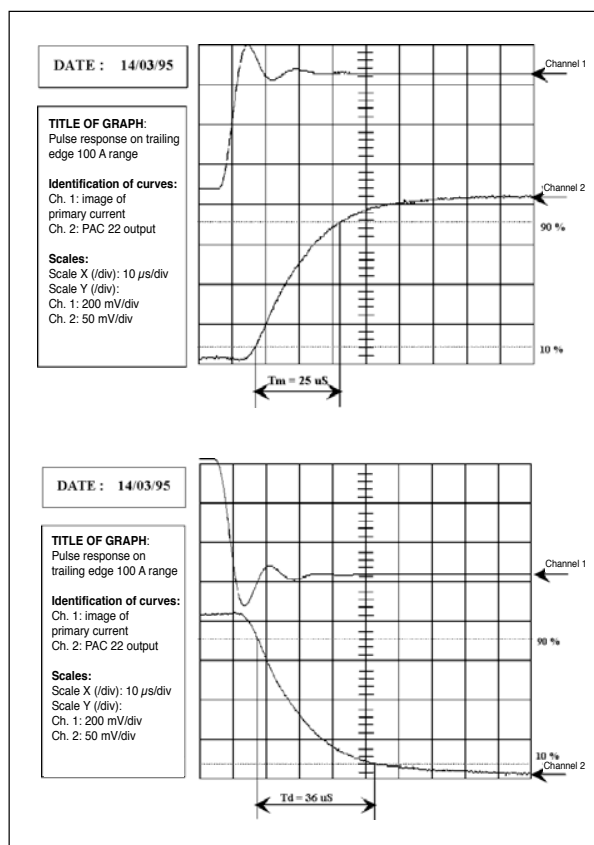
Pulse response
