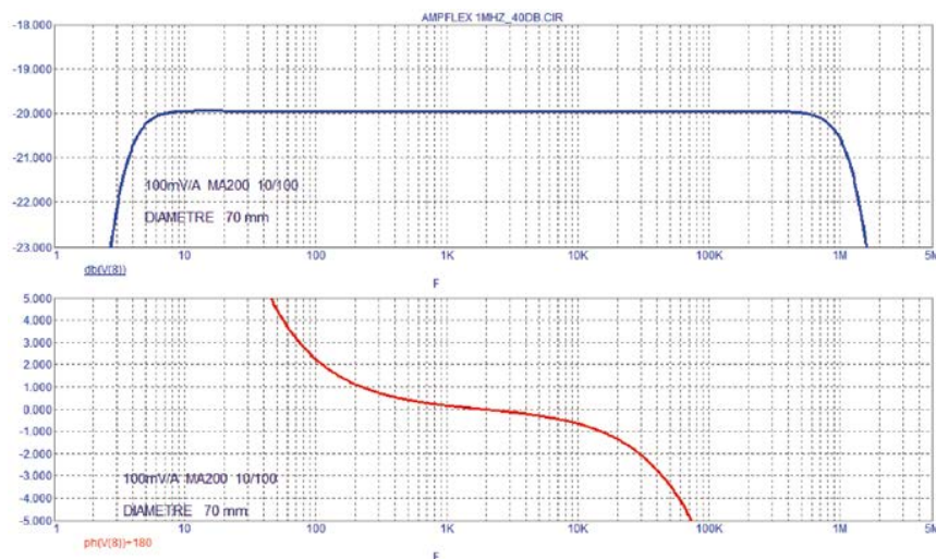
Frequency and phase responses (9)
