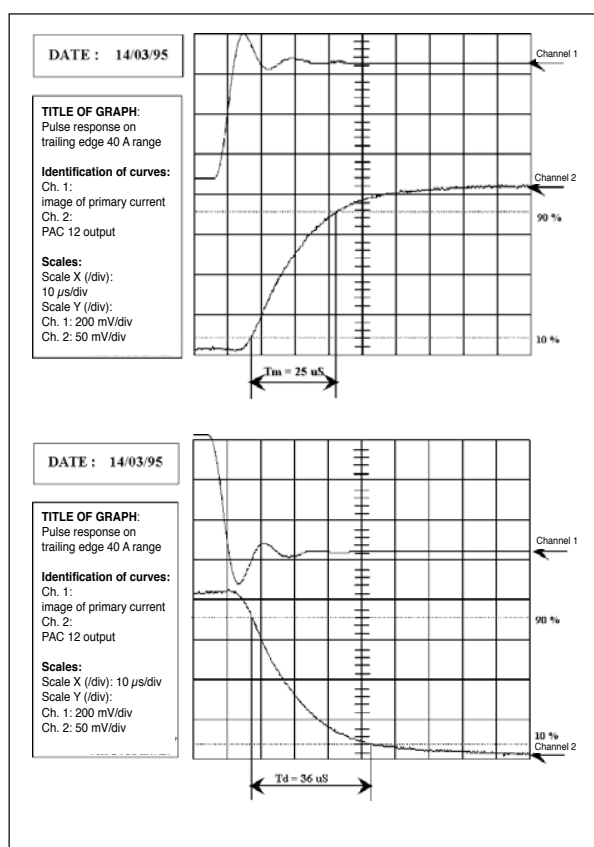
Pulse response
