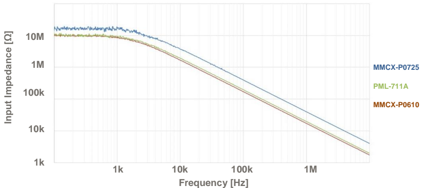
Typical Differential Input Impedance – MMCX-P0725, MMCX-P0610(RO)
