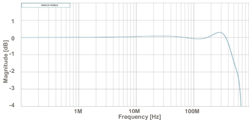
Typical Frequency Response – MMCX-P0610 - normalized
