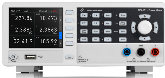
R&S®NPA101
