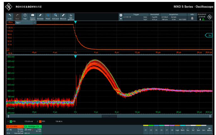
Measurement of a voltage overshoot on a 160 A load step with the A/B/R sequence trigger in MXO. The overshoot varies, depending on the position of the load transient inside the switching cycle of the multiphase buck converter (courtesy Signal Edge Solutions)
