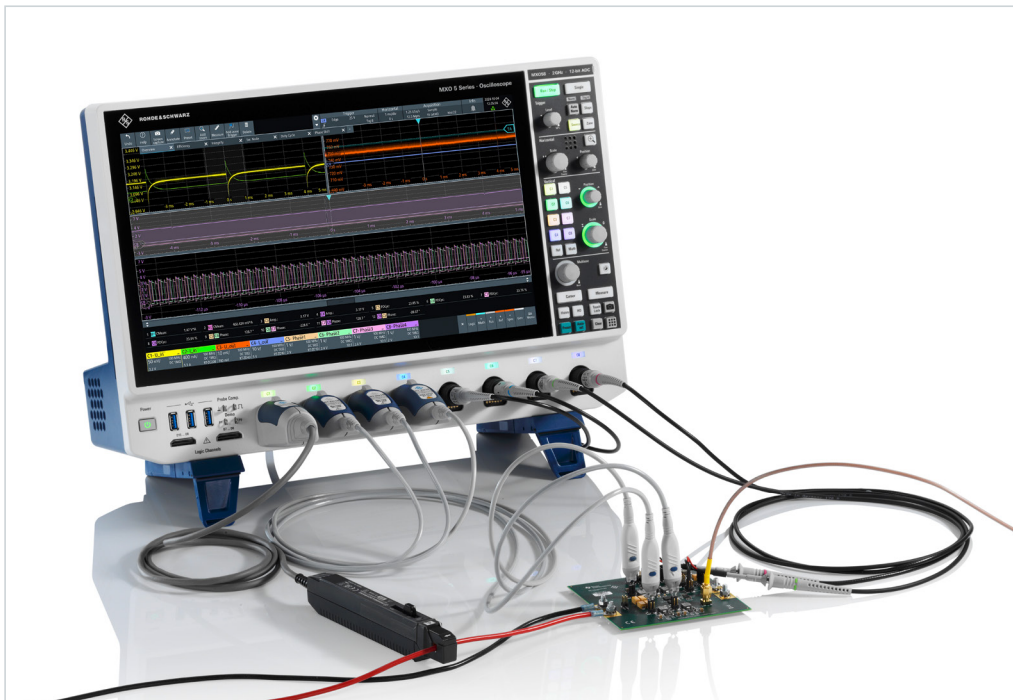
Power integrity analysis of a multiphase buck converter design with an MXO 58 8-channel oscilloscope (courtesy Texas Instruments)
