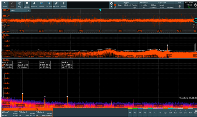
Power integrity analysis in time and frequency domain, showing the 2.24 MHz switching frequency and its harmonics
