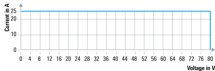
Keysight N6974A
